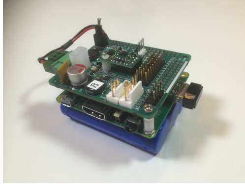
Figure 8: Raspberry Pi with hat board design on top and battery mounted below.
