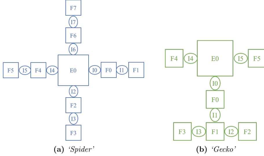
Figure 5: Schematic diagram of two robot morphologies with core component (labelled E0), active hinges (Ix), and fixed bricks (Fx). Full listings of the respective genomes are provided in Appendix B (listings 1 and 2).
