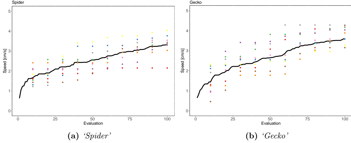
Figure 7: Development of locomotion speed for two robot shapes over 10 replicate runs. The coloured dots denote individual runs, the black curve indicates the average of all 10 runs.
